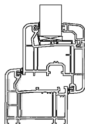
option 5-ch. Uf: 1.3W/m 2 K
