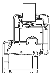
standard 3-ch. Uf: 1.4 W/m 2 K
